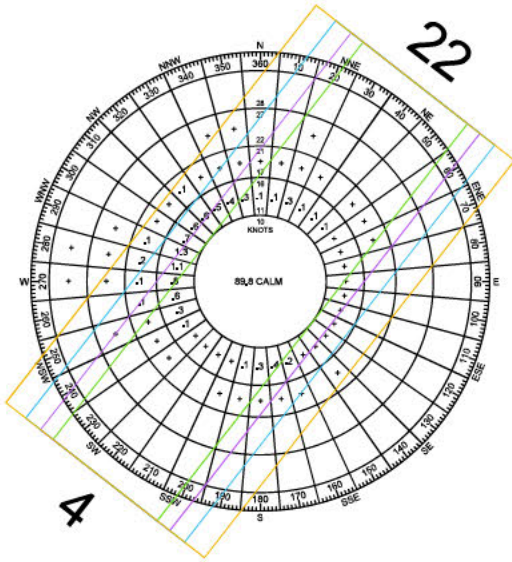
IFR WIND COVERAGE
