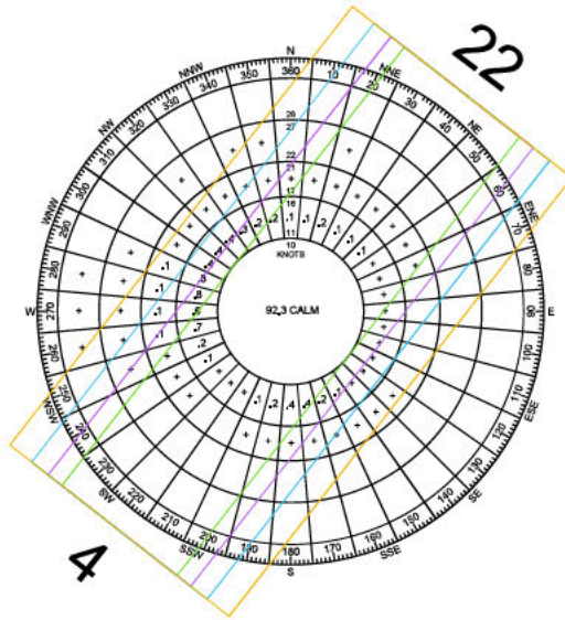
ALL WEATHER WIND COVERAGE
