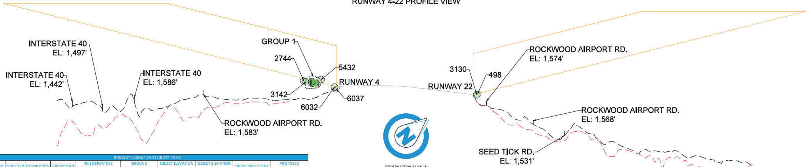
RUNWAY 4-22 PROFILE VIEW
